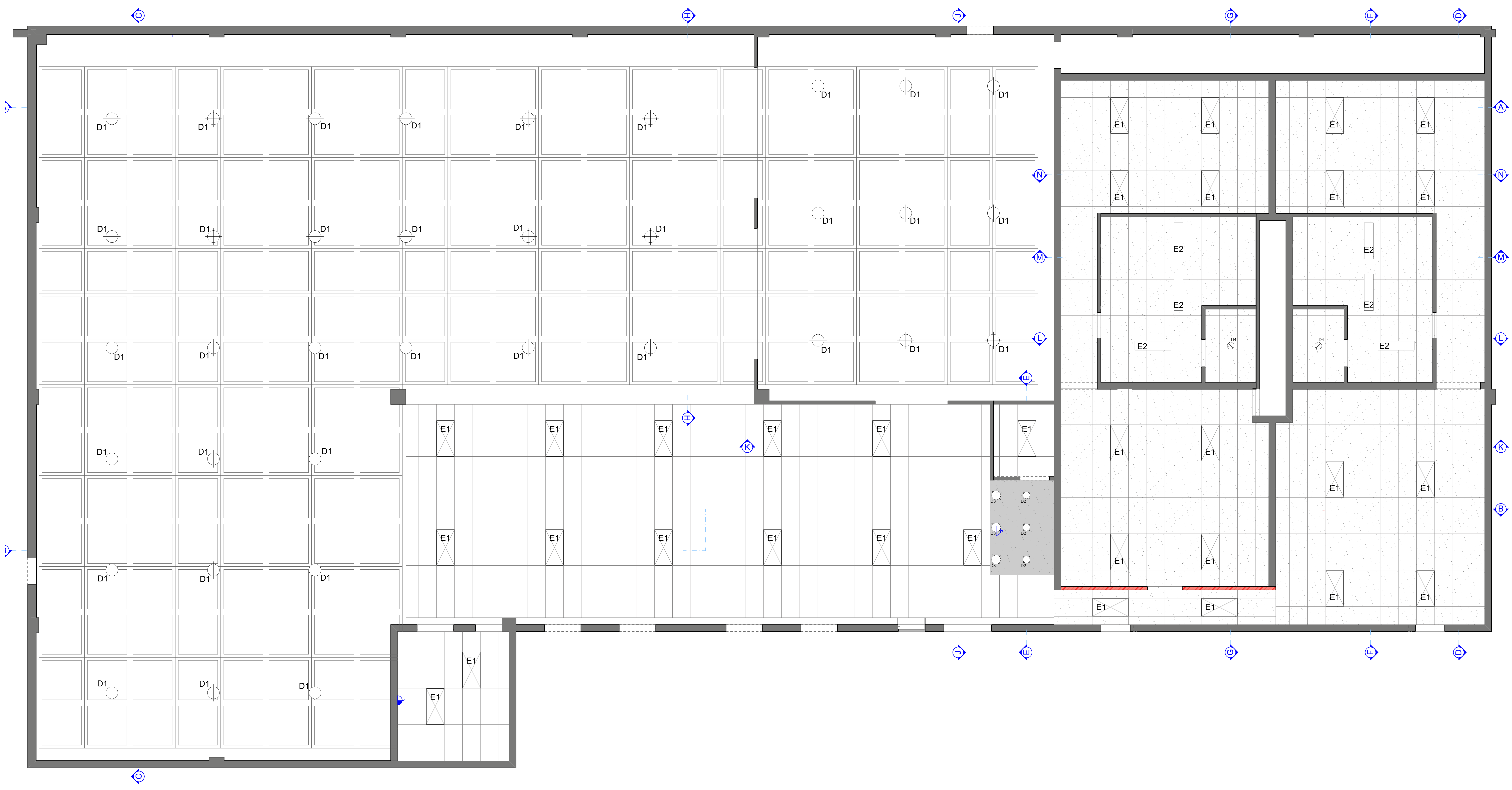
0. Ceiling Layout Plan 1:50
